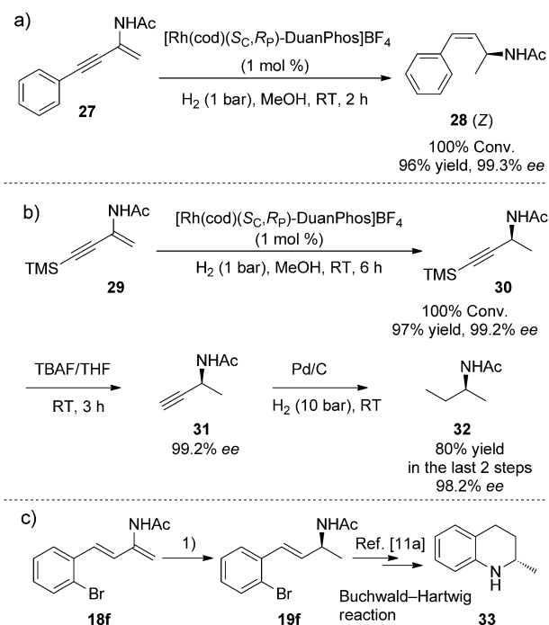
Scheme 3. a) Synthesis of Z -allylic amine 28 . b) Synthesis of ( S )-but-3-yn-2-amine 31 and ( S )-butan-2-amine 32 . TMS = trimethylsilyl, TBAF = tetrabutylammonium fluoride. c) Catalytic enantioselective synthesis of 2-methyl-1,2,3,4-tetrahydroquinoline ( 33 ) starting from 19f . Reaction conditions: 1) [Rh(cod)(S C , R P )-DuanPhos]BF 4 , 1 bar H 2 , MeOH, RT, 2 h.
